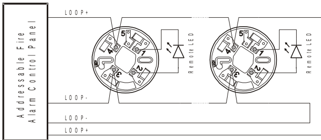
Figure 1. Wiring diagram:
